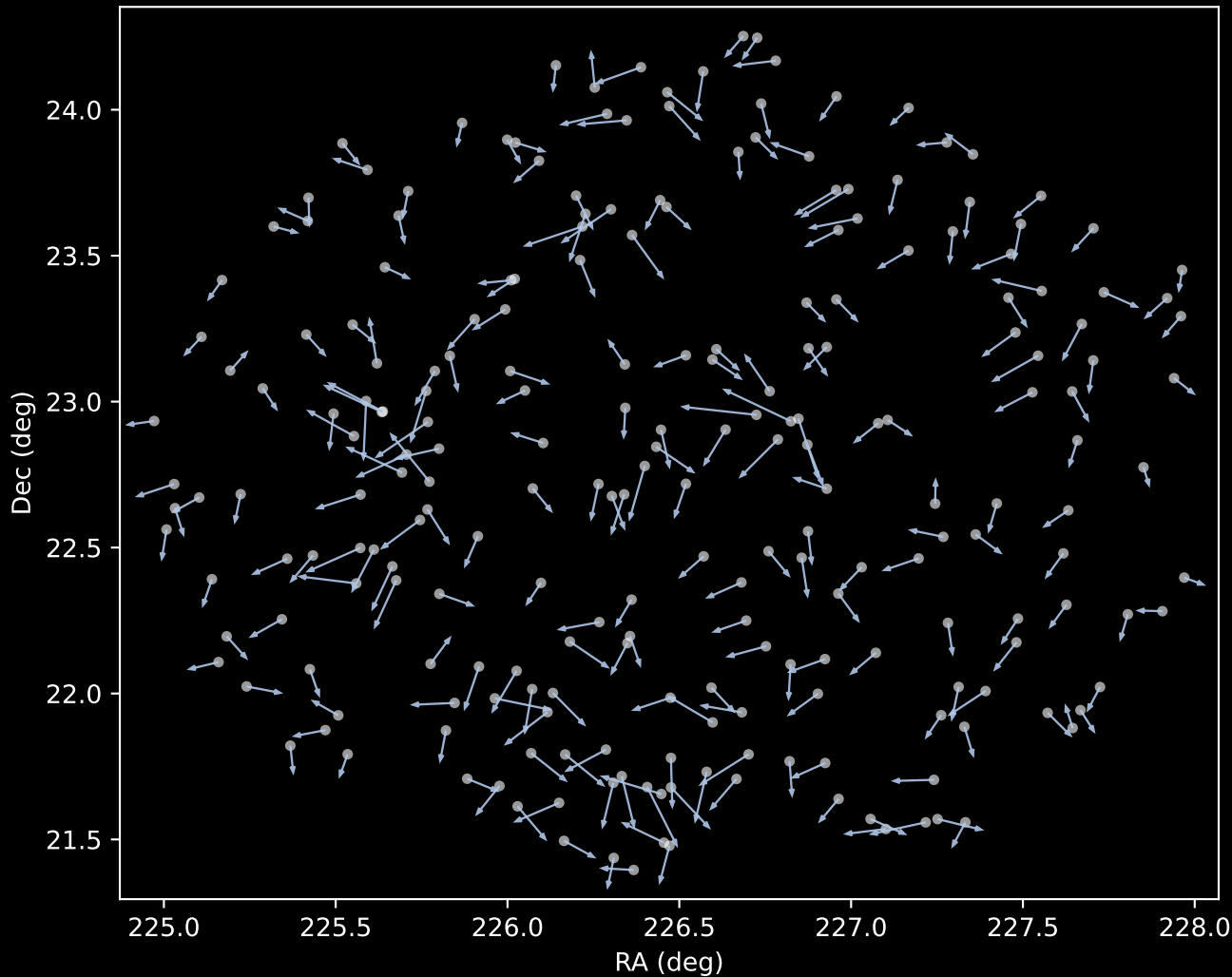
APOGEE DR17 Cluster 1 Proper Motion Vectors (n=232)
