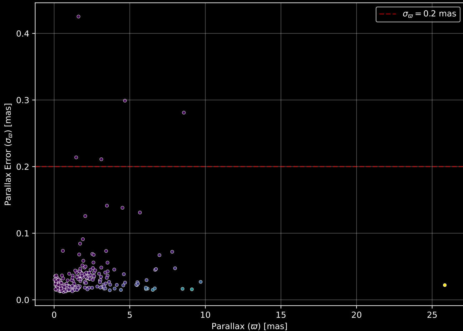
APOGEE DR17 Field: [201+30_btx] Parallax Quality (n= 297)
