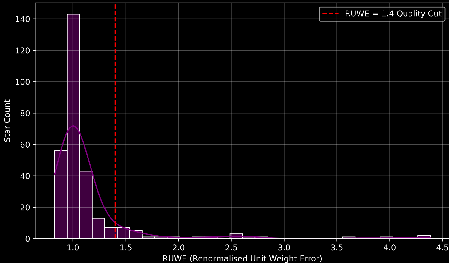
GAPOGEE DR17 Field [201+30_btx] RUWE Distribution (n= 288)
