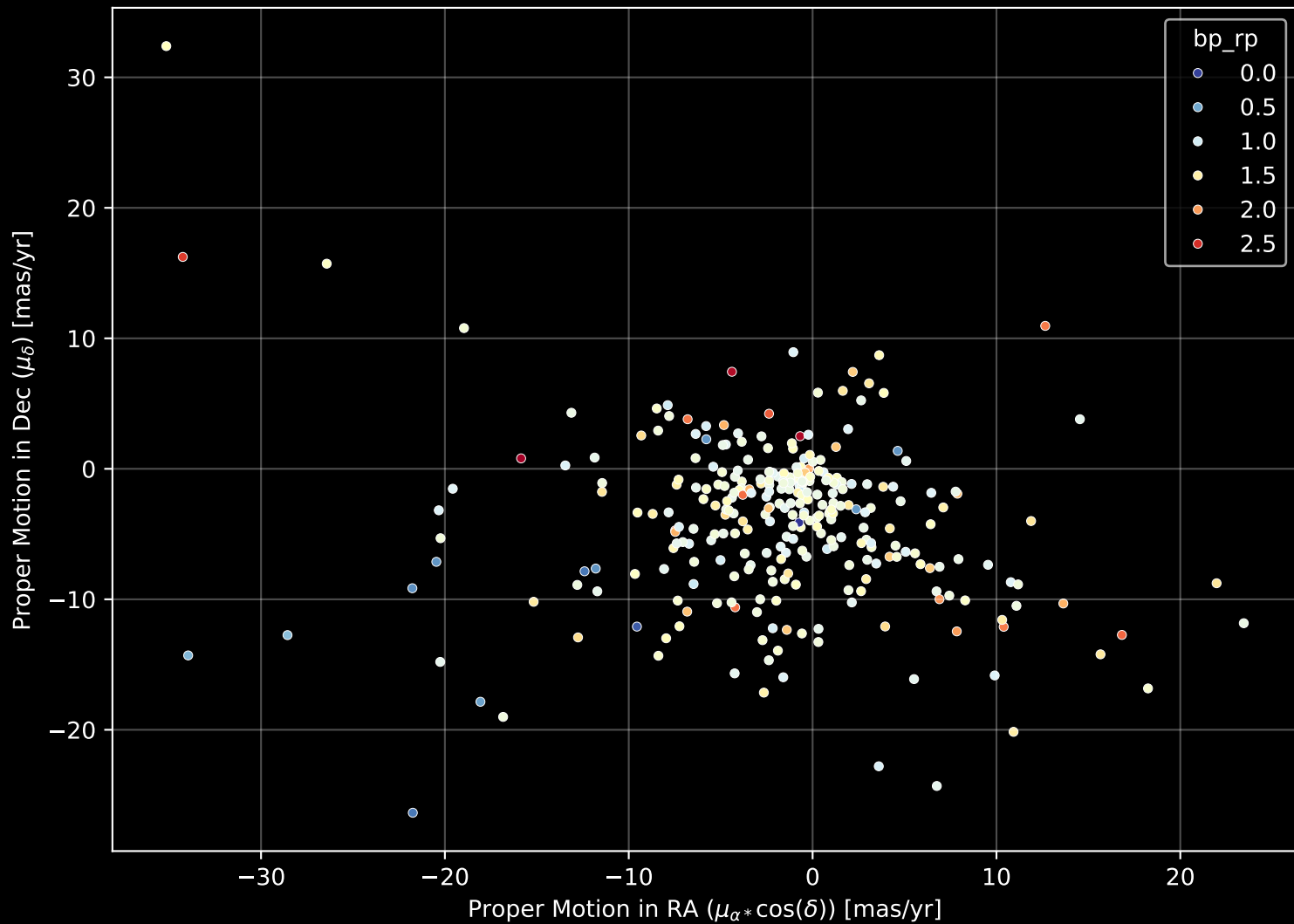
APOGEE DR17 Field: [201+30_btx] Proper Motion Diagram (n= 297)
