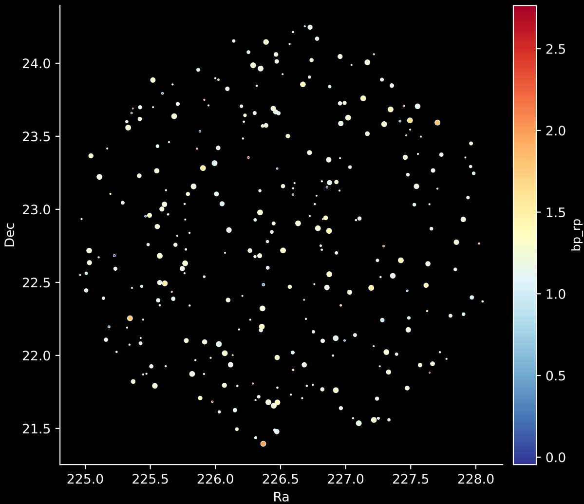
APOGEE DR17 Field: [201+30_btx] Stars: 297
