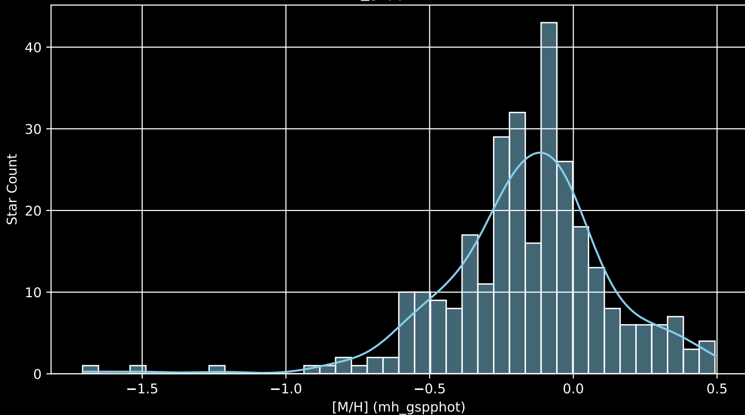
APOGEE DR17 Field: [201+30_btx [M/H] (mh_gspphot) (n= 294)
