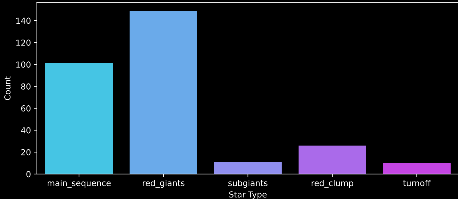
APOGEE DR17 Field: [201+30_btx] Count plot of Star Type
